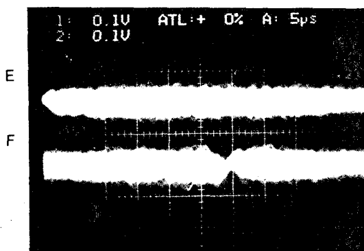
The two beam are on the same pit line. (100mV/DIV : 5\mu s /DIV)
