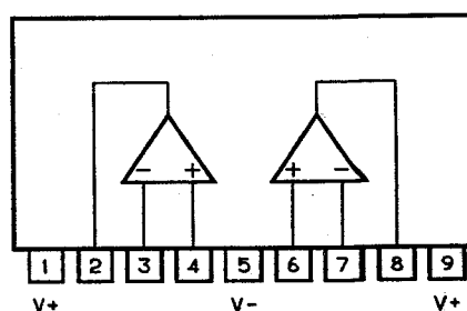
NJM2068/NJM2903S BLOCK DIAGRAM
